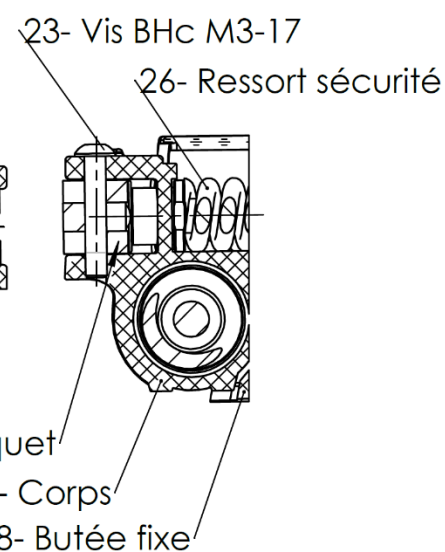
Coupe H-H locale
